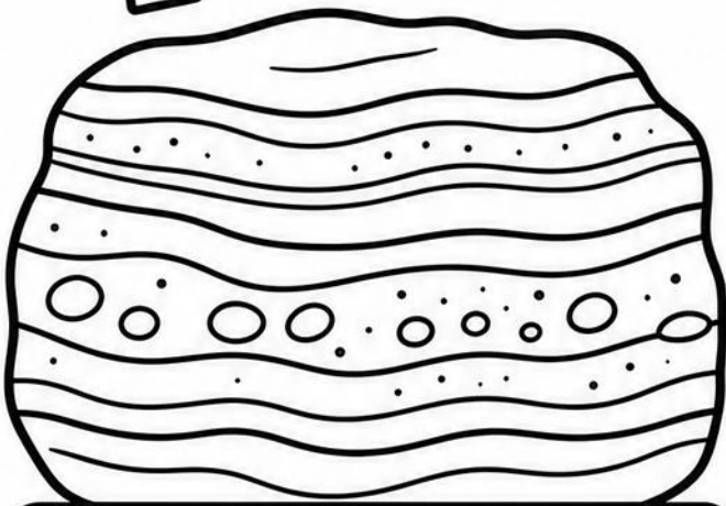
SEDIMENTARY ROCK
