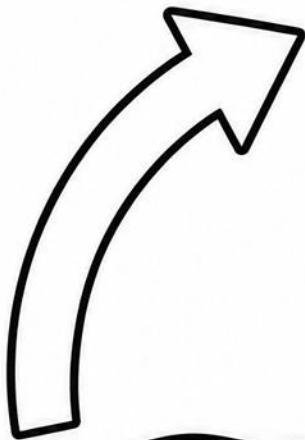
IGNEOUS ROCK
