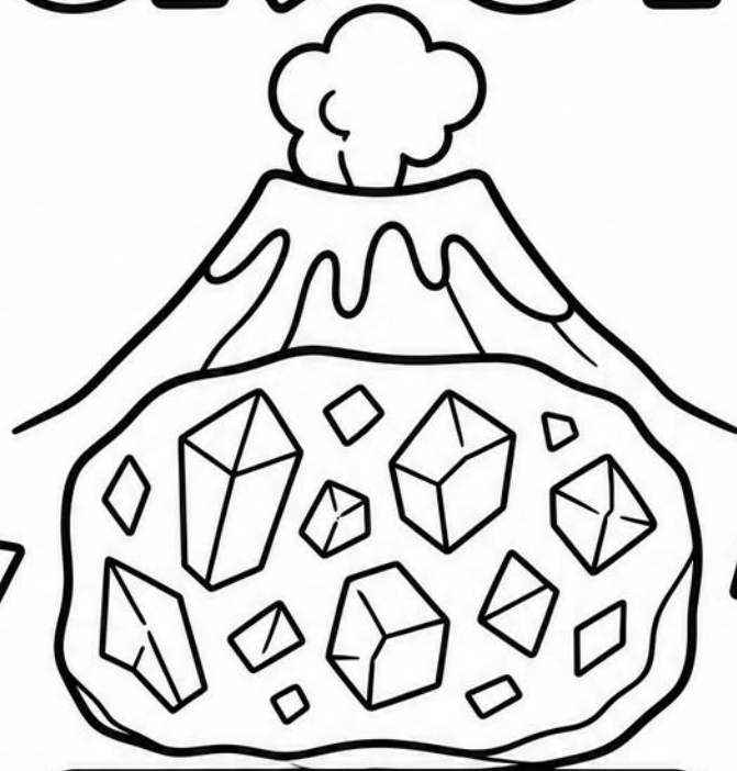
IGNEOUS ROCK
