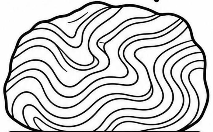
METAMORPHIC ROCK
