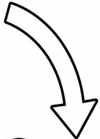
IGNEOUS ROCK
