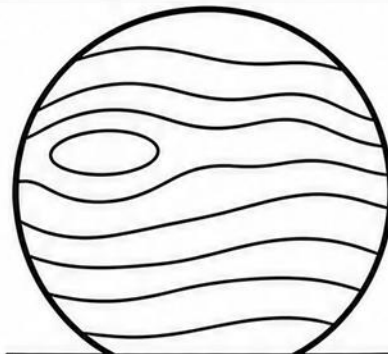
NEPTUNE
