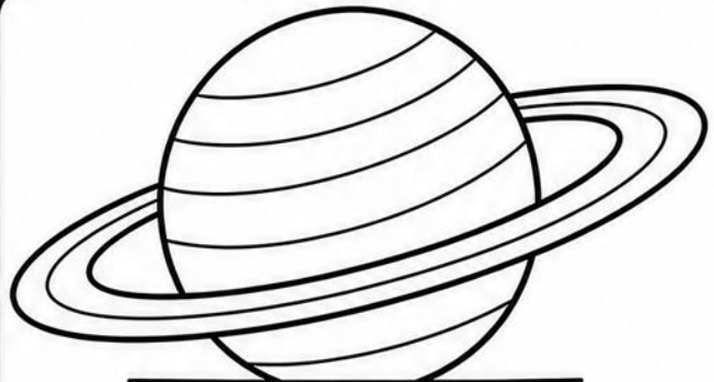
SATURN
