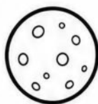
MERCURY
