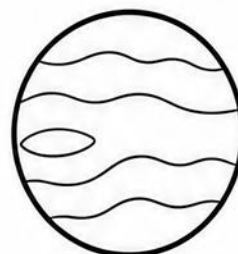
NEPTUNE
