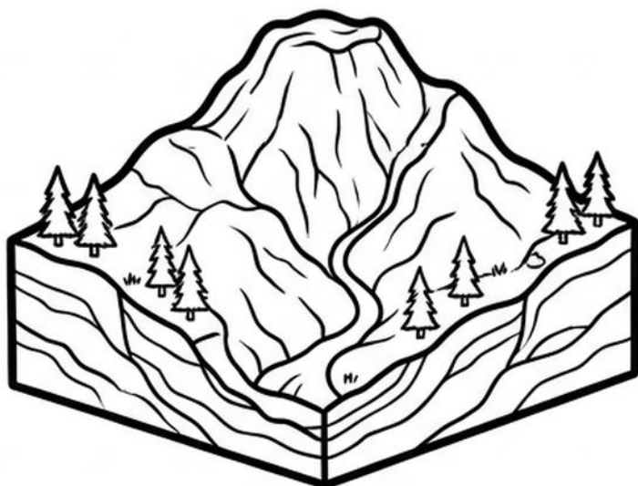
4. ERODED PEAK
