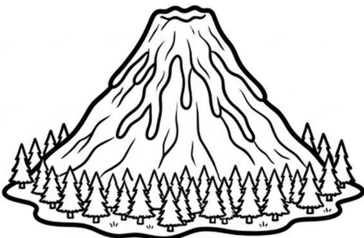
2. GROWTH & COOLING
