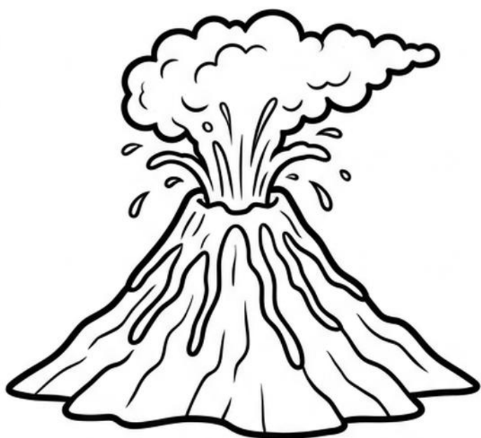
1. VOLCANIC ERUPTION
